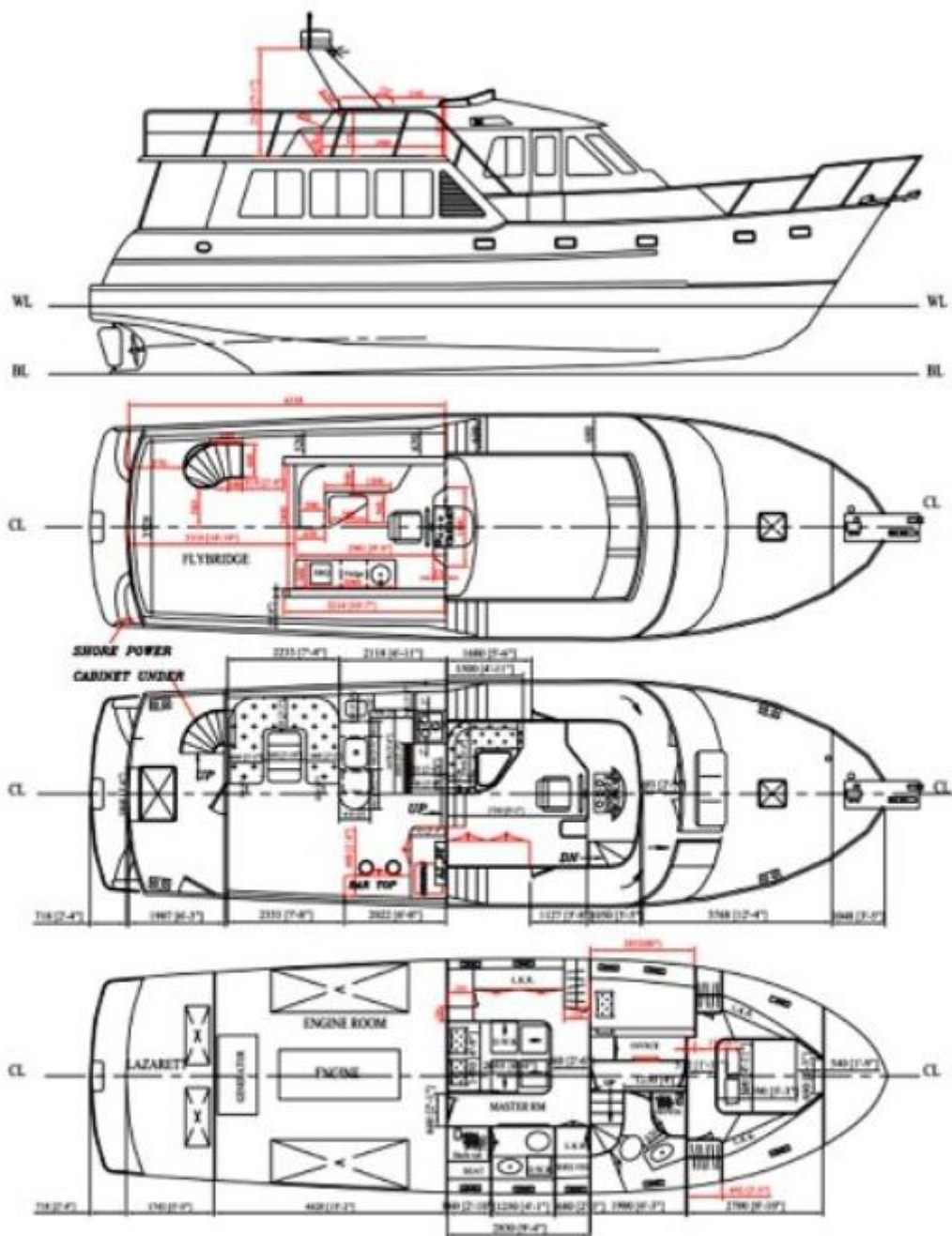
Floor Plan - 3 staterooms
